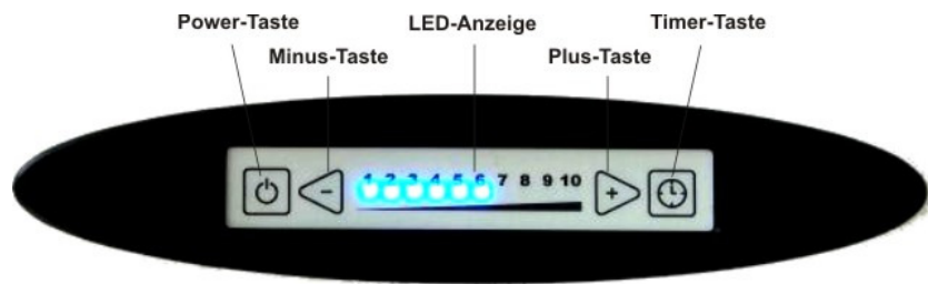
[Abb. 2: Bedienfeld]
