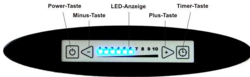
[Abb. 2: Bedienfeld]
